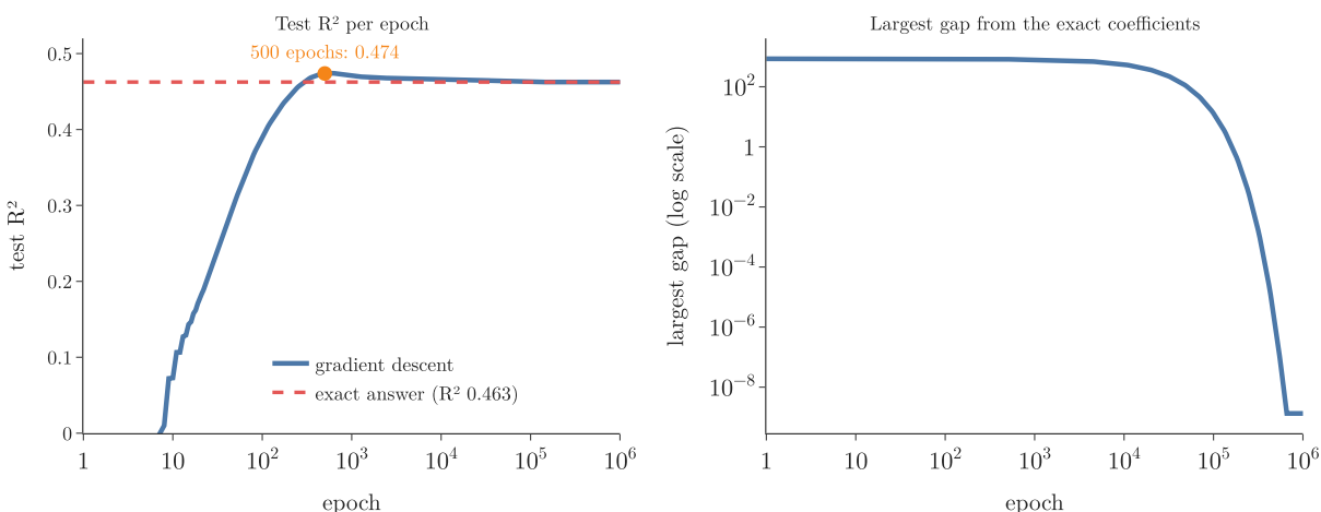
Figure 4: Test R^2 and distance from the exact answer, per epoch
