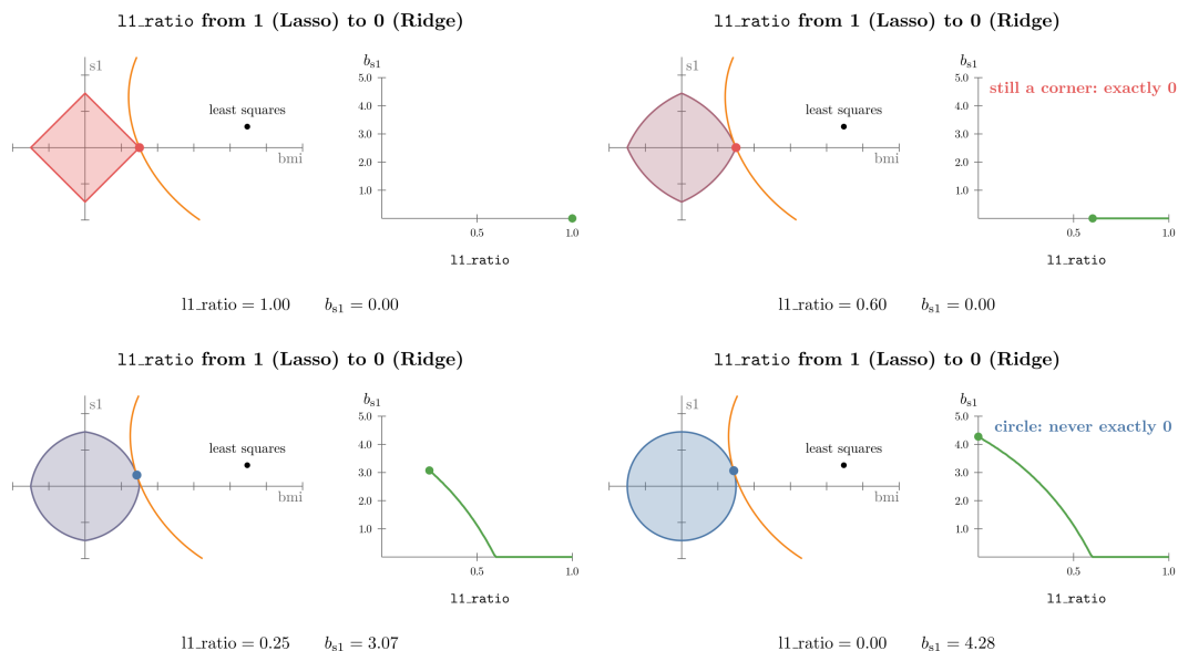
Figure 2: The allowed region morphs from Lasso’s diamond ( l1\_ratio 1) to Ridge’s circle ( l1\_ratio 0) on two diabetes features. The s1 coefficient, where the loss ellipse first touches the region, stays exactly 0 down to l1\_ratio 0.6 and then grows to 4.28
