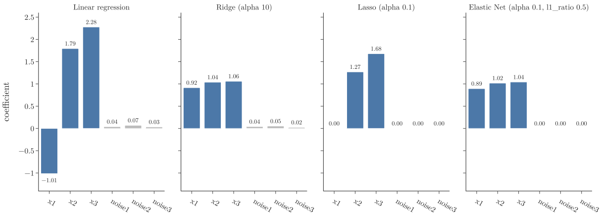
Figure 3: Coefficients of four models on three correlated inputs and three noise inputs
