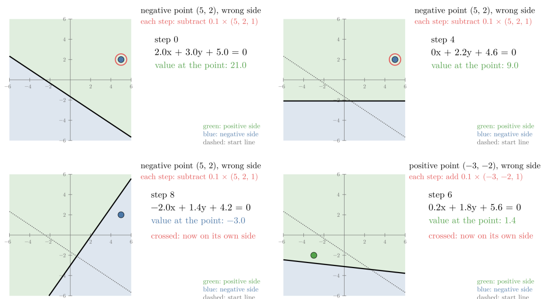
Figure 5: The perceptron trick in small steps, learning rate 0.1. First, the negative point (5, 2) sits on the positive (green) side; each step subtracts 0.1 \times (5, 2, 1) from the coefficients, its value falls by 3 (21, 18, 15, ...), and at step 8 the point is on the negative side. Then the positive point (-3, -2); each step adds 0.1 \times (-3, -2, 1) , its value rises by 1.4 from -7, and it crosses at step 6. The dashed line is the start line 2x + 3y + 5 = 0
