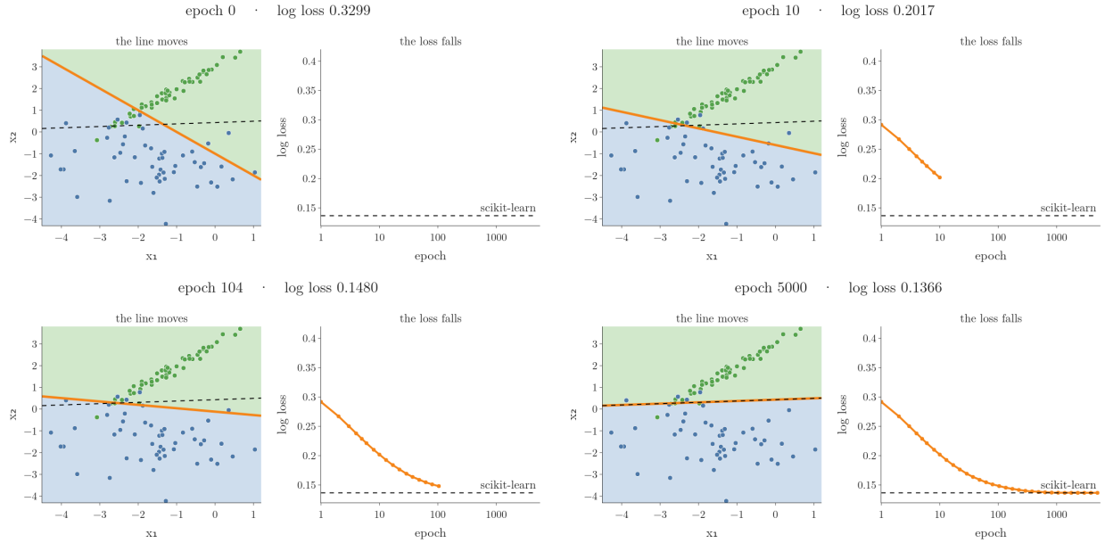
Figure 2: Batch gradient descent on the 100 points. Left: the line where p = 0.5 turns into place; the dashed line is scikit-learn's. Right: the log loss per epoch (log scale) falls to scikit-learn's minimum.
