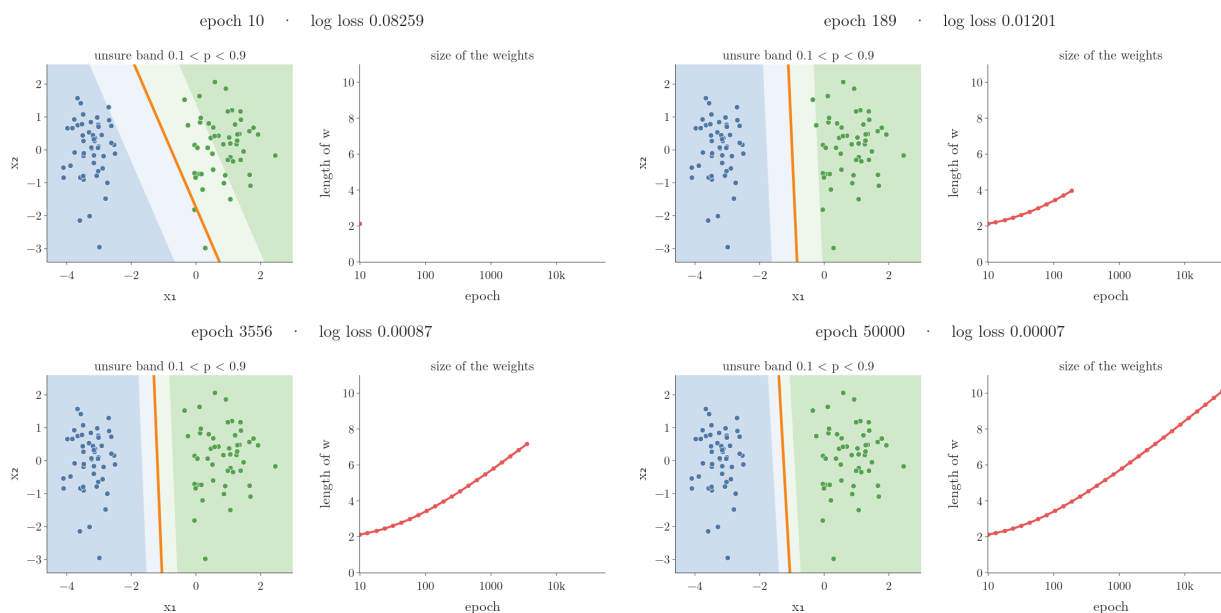
Figure 3: Batch gradient descent on perfectly separated points. Left: the pale band is where the model is unsure ( 0.1 < p < 0.9 ); the orange line is p = 0.5 . Right: the length of the weight vector per epoch (log scale).
