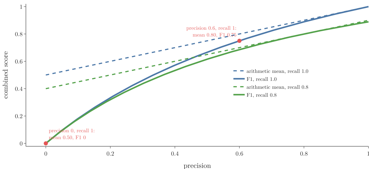
Figure 3: F1 against the arithmetic mean
