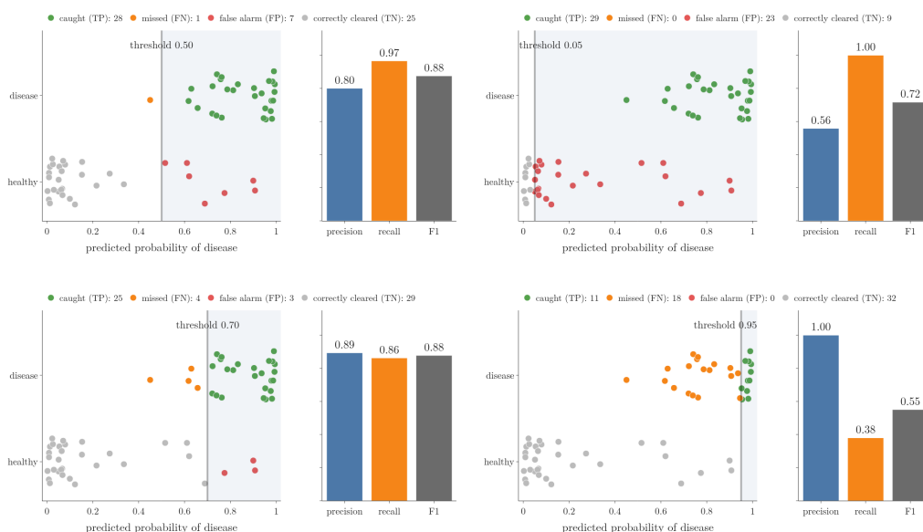
Figure 2: The decision threshold slides across the heart-disease test set. Each dot is a patient at its predicted probability of disease, in the lane of its true class; the shaded side is flagged. Green: caught; orange: missed; red: false alarm; grey: correctly cleared. Right: precision, recall and F1 at that threshold
