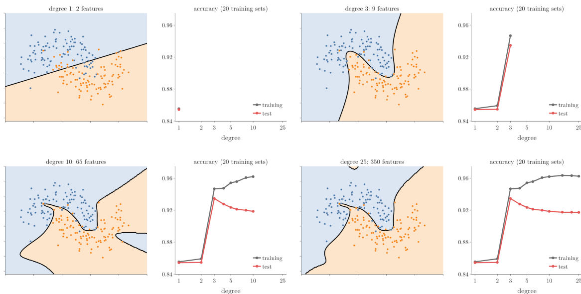
Figure 1: Degree swept from 1 to 25. Left: decision regions for one training set (black line: the boundary). Right: training and test accuracy, averaged over 20 training sets
