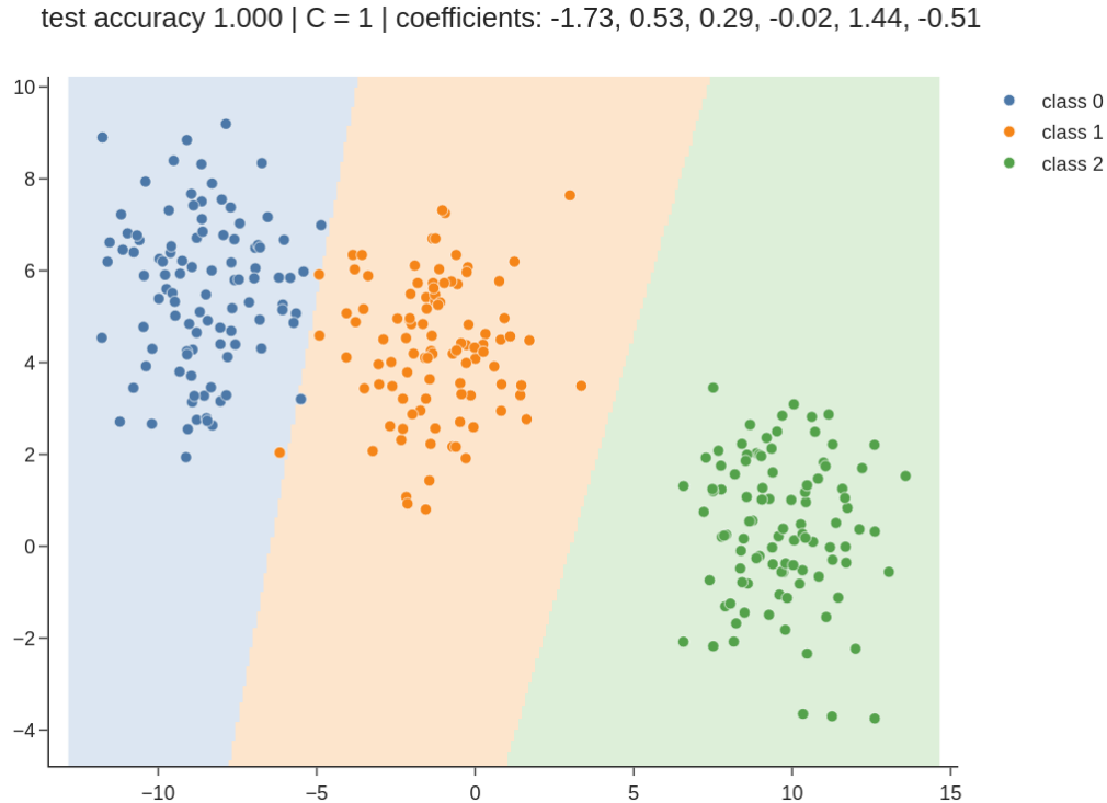
Figure 3: The playground on the three-class dataset with the default settings
