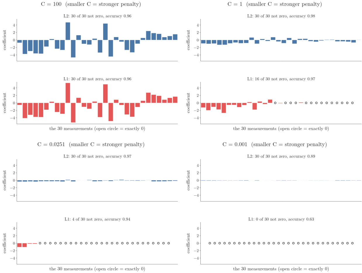
Figure 2: The 30 coefficients on the breast-cancer data as C falls from 100 to 0.001, for L2 (top) and L1 (bottom); titles give the 5-fold CV accuracy
