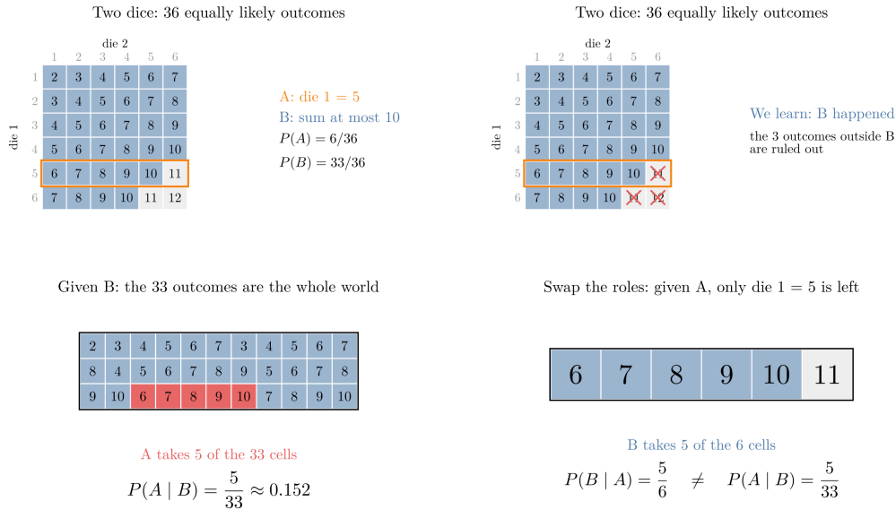
Figure 3: Conditioning shrinks the sample space: the 3 outcomes outside B are ruled out, the 33 left become the whole world and A covers 5 of them; given A instead, B covers 5 of A's 6 outcomes
