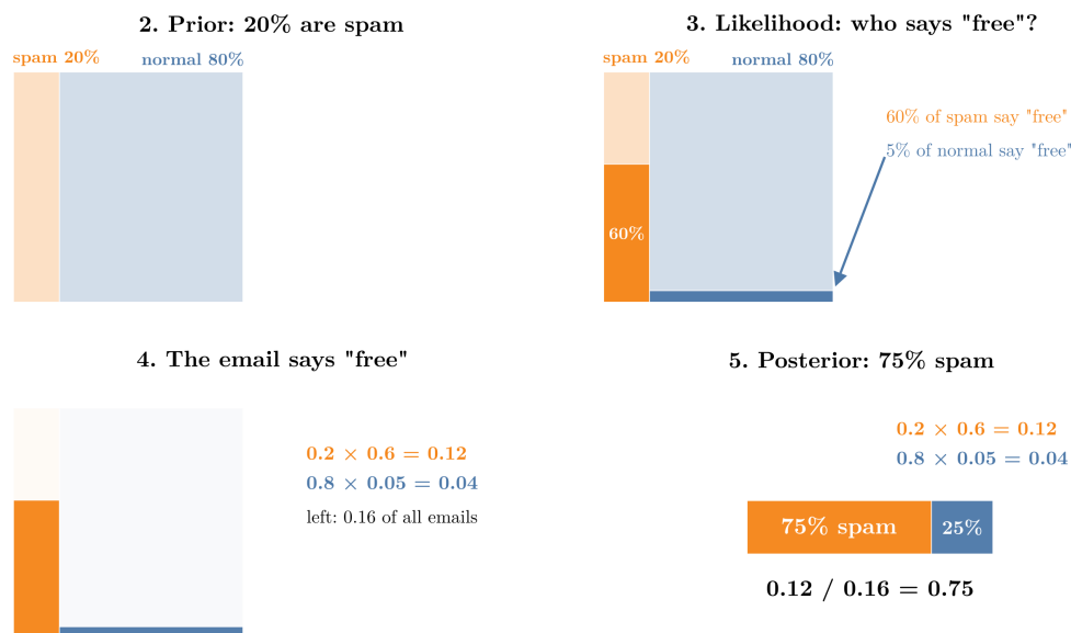
Figure 2: Bayes’ theorem as areas. Prior: a 20% spam strip. Likelihood: the “free” share inside each strip. Evidence: only the two dark pieces remain (0.12 and 0.04). Posterior: rescaled to fill the whole, spam is 0.12 / 0.16 = 75\% . Picture after Sanderson (3Blue1Brown), “Bayes’ theorem”.
