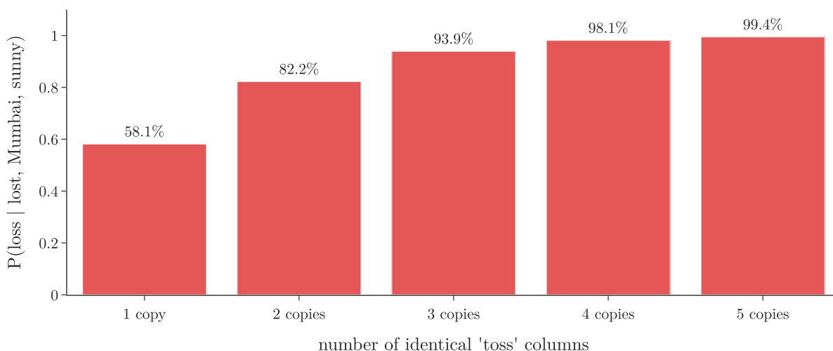
Figure 4: Copying a feature makes Naive Bayes over-confident
