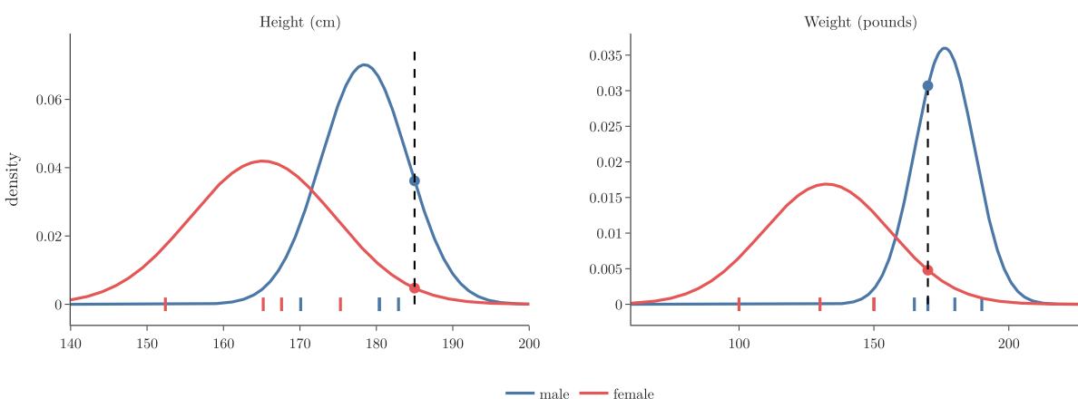
Figure 1: A normal curve per class for each feature; the dots mark the new person's values
