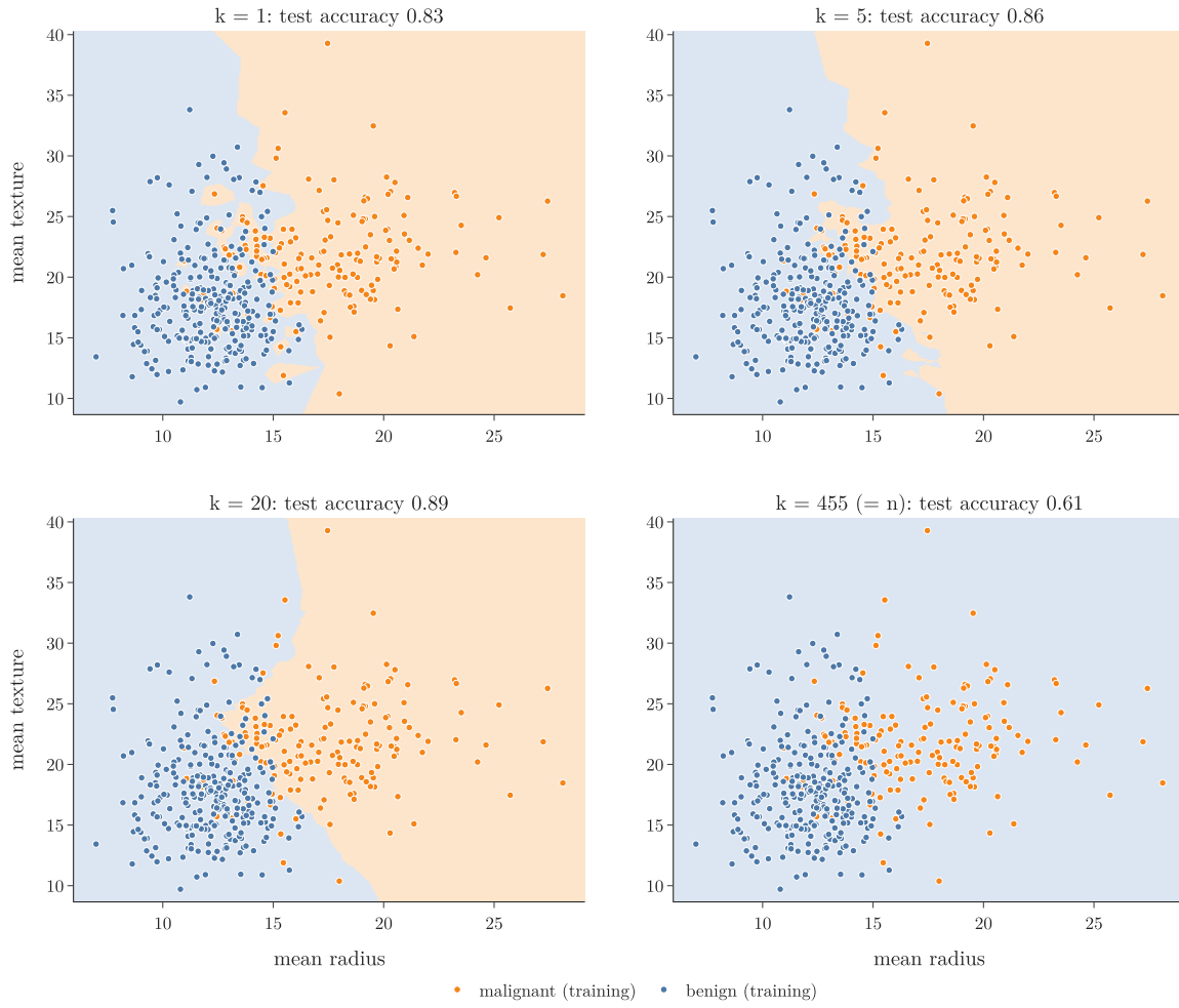
Figure 4: Decision surfaces for k = 1, 5, 20 and k = n = 455 , with test accuracy on the same two features
