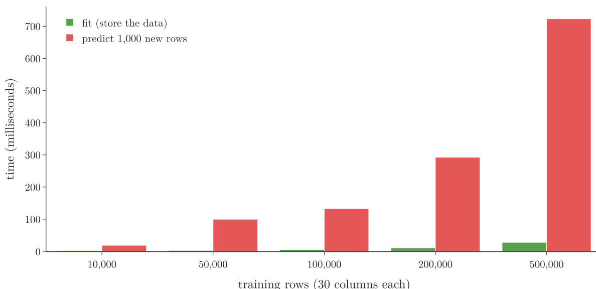
Figure 6: Fit time and prediction time of KNN (brute-force search) as the training set grows
