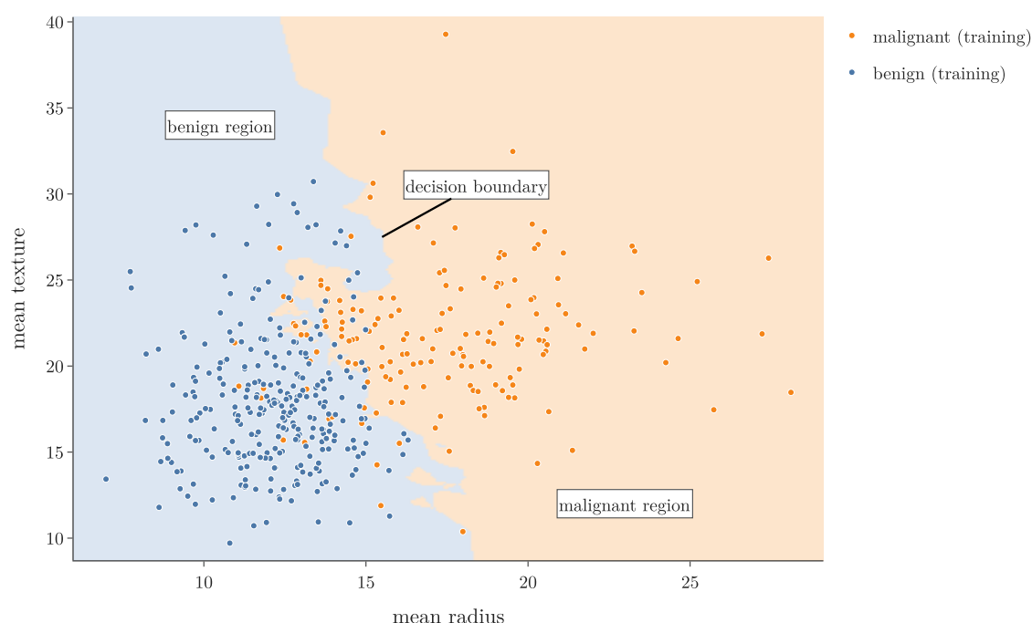
Figure 3: KNN ( k = 5 ) on two breast cancer features: the decision regions and the decision boundary
