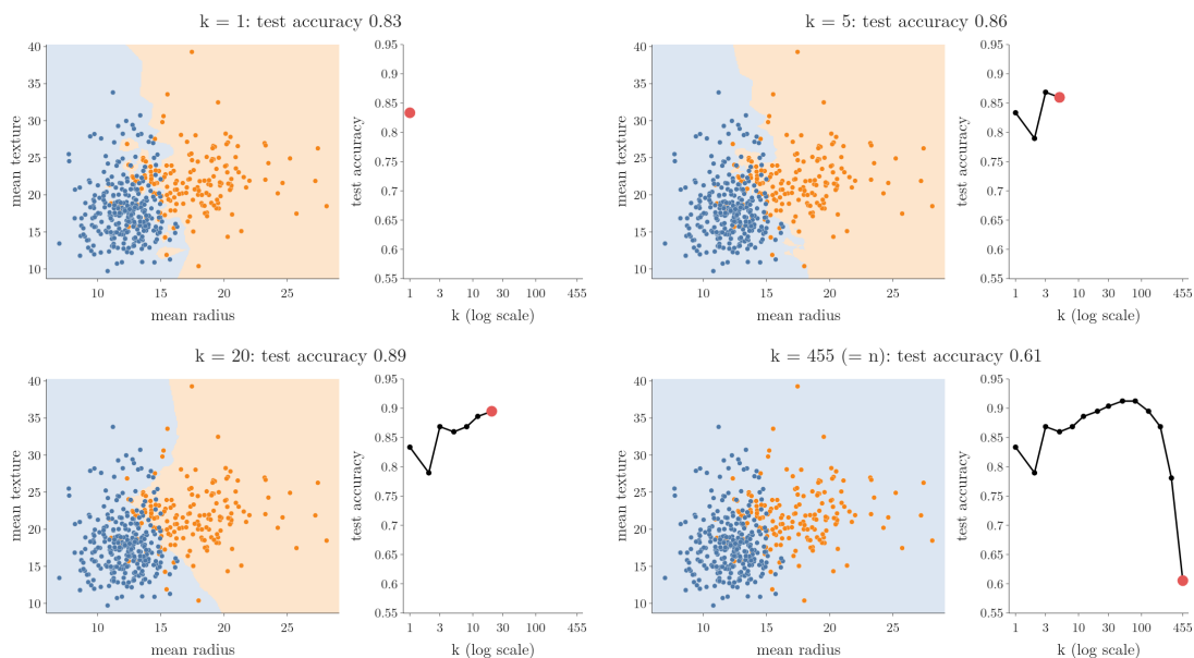
Figure 5: k swept from 1 to n = 455 on the same two features: the decision surface (left) and the test accuracy so far (right)
