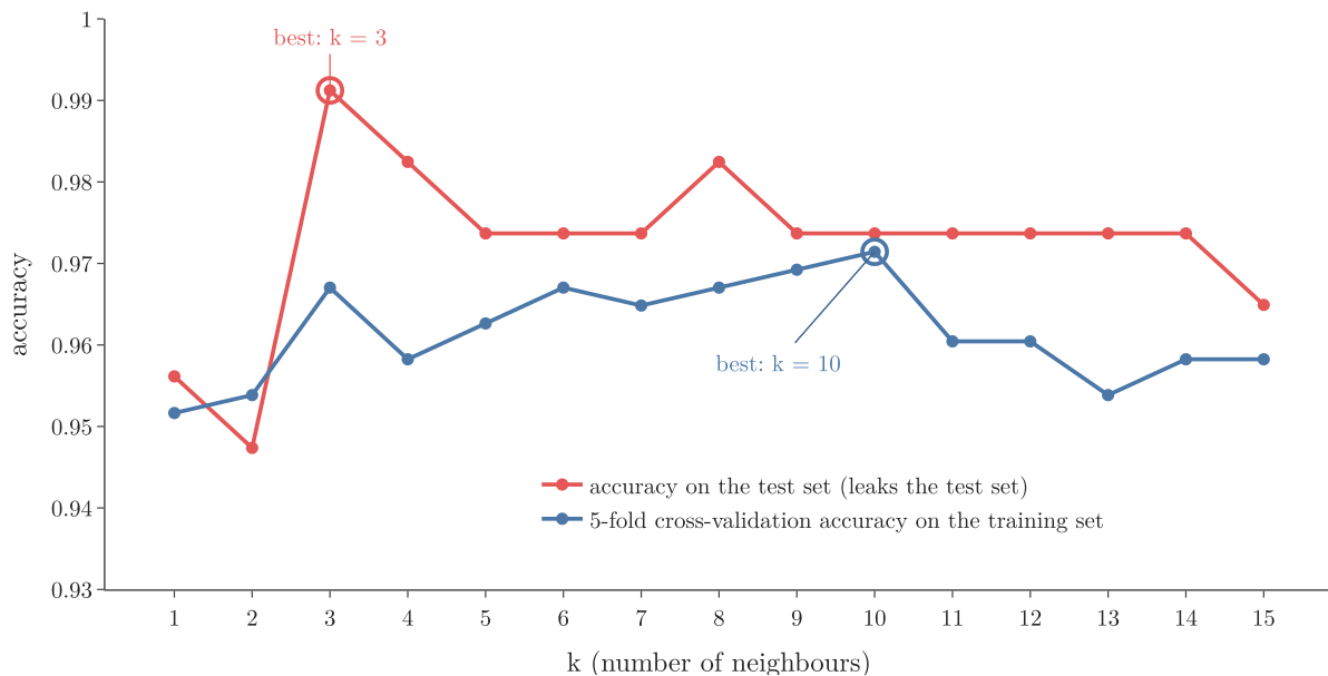
Figure 2: Accuracy against k on the breast cancer data. Red: scored on the test set. Blue: 5-fold cross-validation on the training set
