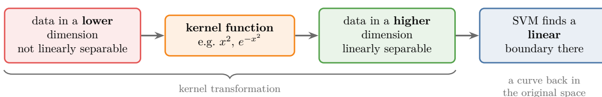
Figure 1: The kernel trick: lift data that is not linearly separable into a dimension where it is
