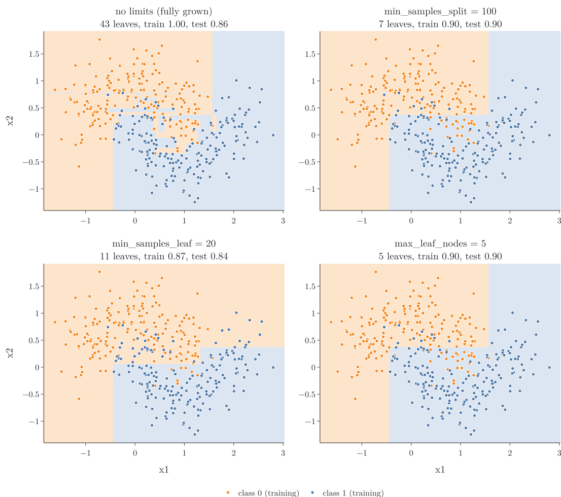
Figure 4: Four ways to stop the tree early on the moons data
