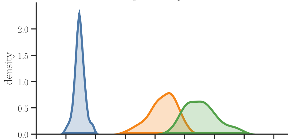
petal length
