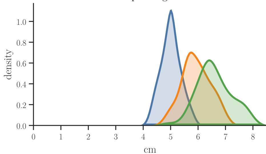
sepal length
