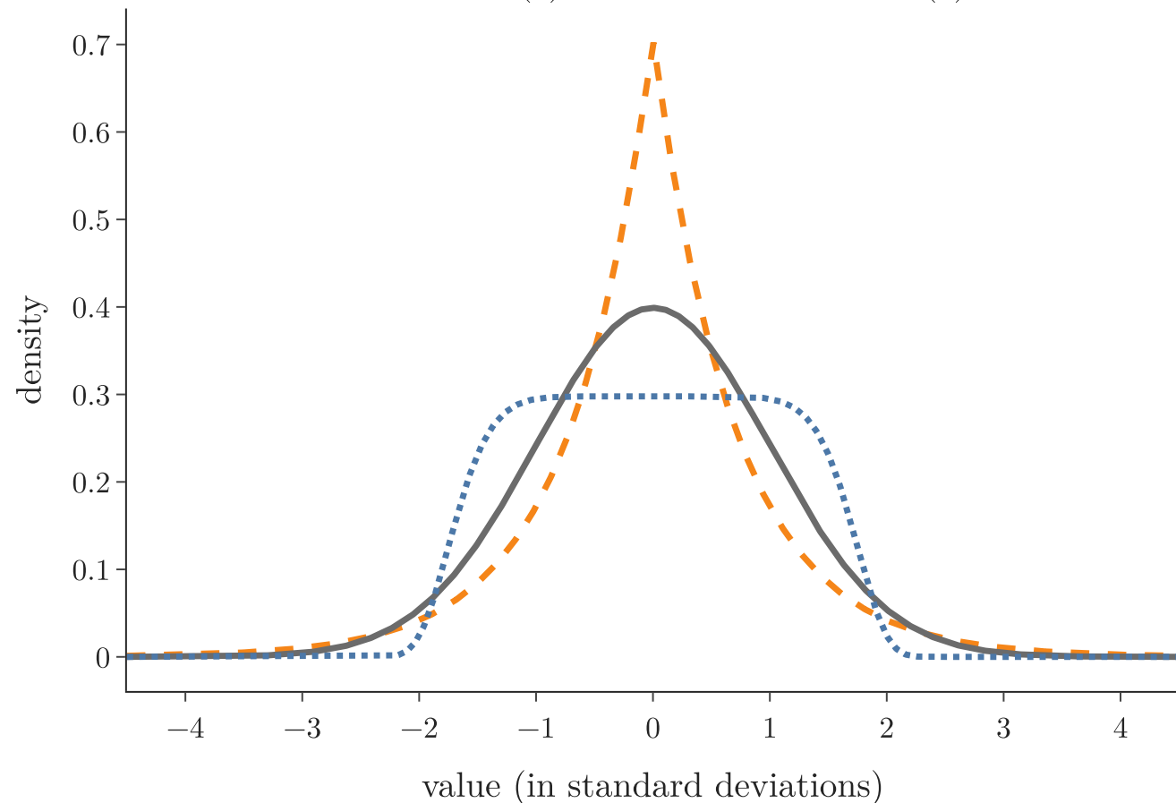
Same mean (0) and standard deviation (1)
