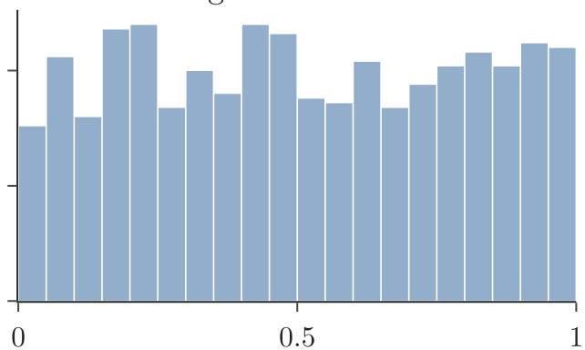
Uniform, thin tails (excess kurtosis -1.2) against normal
