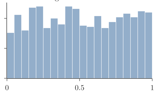
Same uniform data against uniform
