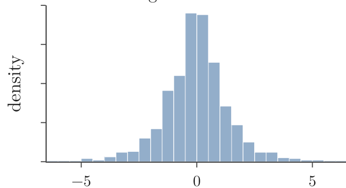
Fat tails (excess kurtosis 2.3) against normal
