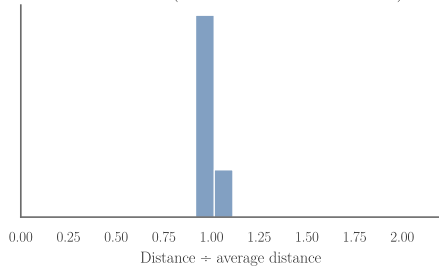
1000 columns (farthest is 1.1\times the nearest)
