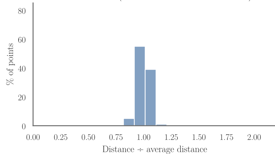
100 columns (farthest is 1.4\times the nearest)
