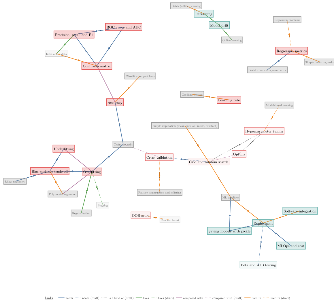
Figure 7: Concept map: Evaluating, tuning and production
