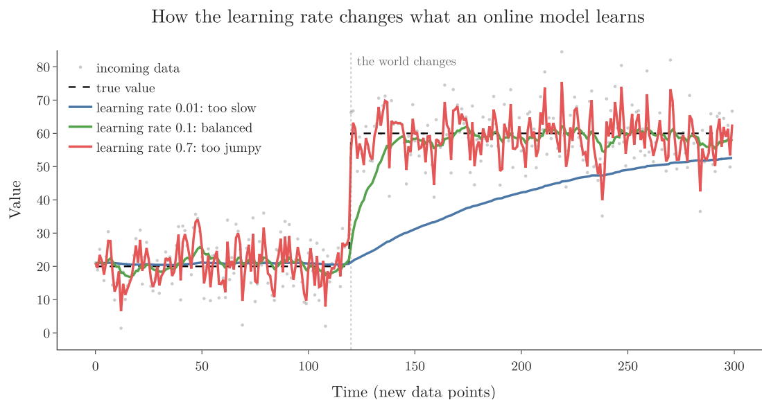
Figure 3: How the learning rate changes what an online model learns
