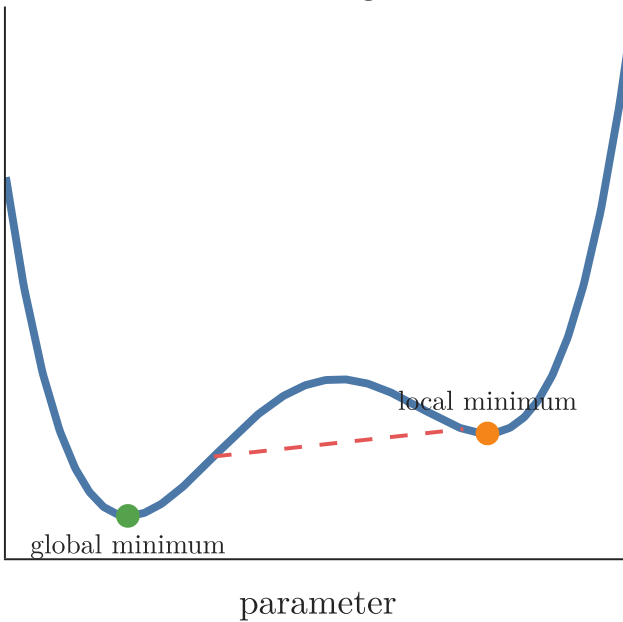
Non-convex: local and global minimum
