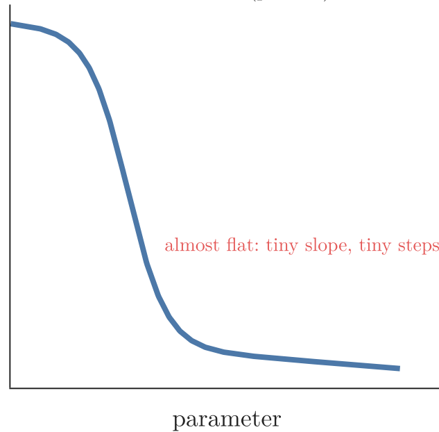
A flat stretch (plateau)
