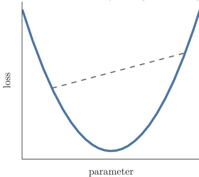
Convex: one minimum (linear regression's MSE)
