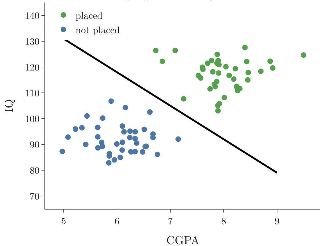
Linearly separable: a straight line works
