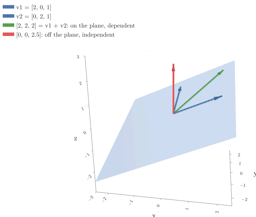
Figure 3: The plane spanned by \mathbf{v}_1 and \mathbf{v}_2 , a third vector on it (green) and one off it (red)
