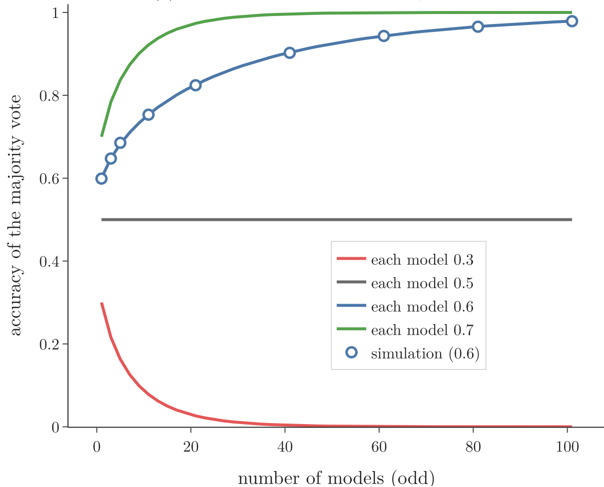
(a) independent models: accuracy of the vote
