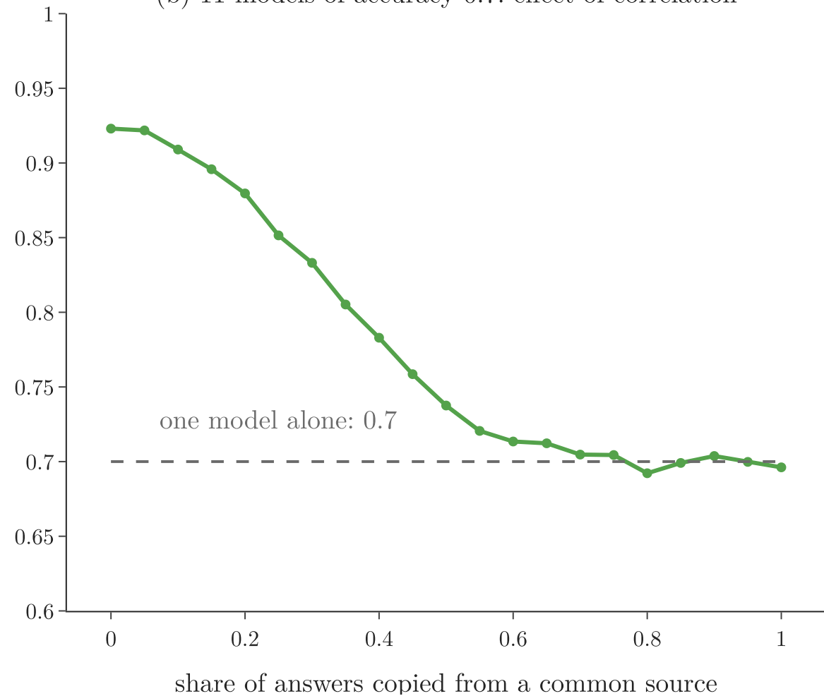
(b) 11 models of accuracy 0.7: effect of correlation
