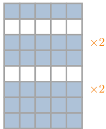
bagging
