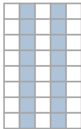
random subspaces
