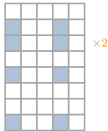
random patches
