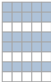
pasting
