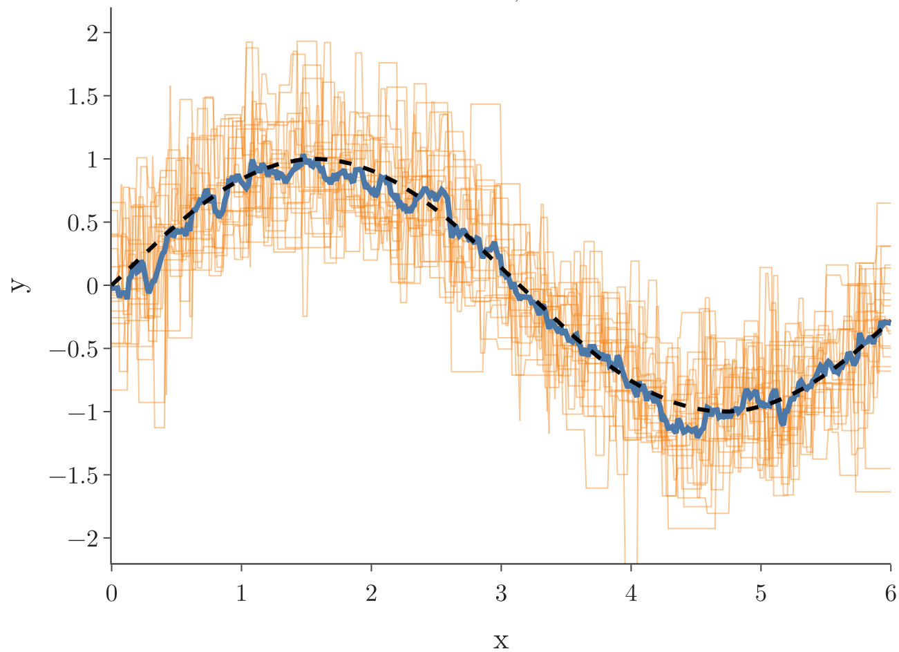
(a) one fully grown tree per training set variance 0.160, bias 2 0.009
