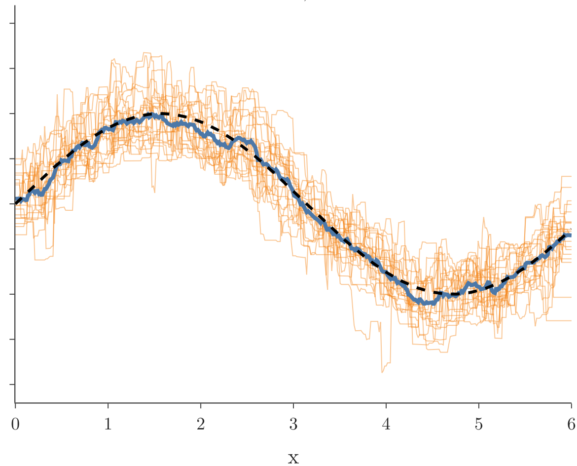
(b) bagging, 100 trees per training set variance 0.076, bias 2 0.004
