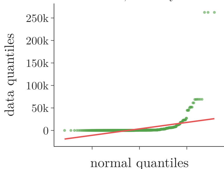
Square: x^2 skew 11.93, accuracy 64.3%
