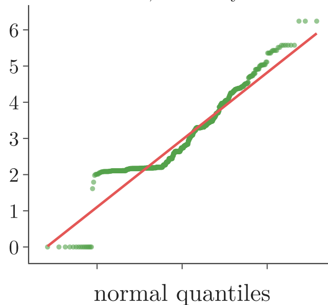
Log: \log(1 + x) skew 0.39, accuracy 67.1%
