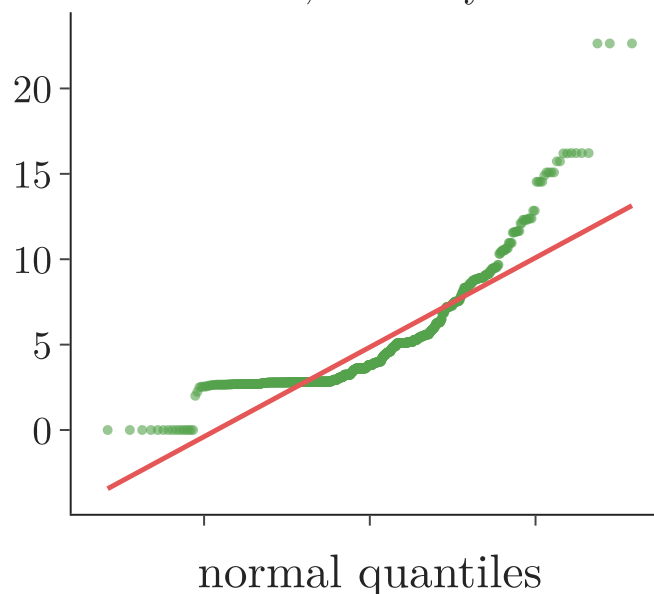
Square root: \sqrt{x} skew 2.09, accuracy 66.1%
