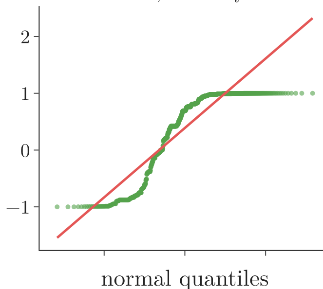
Sine: \sin(x) skew -0.87, accuracy 62.0%
