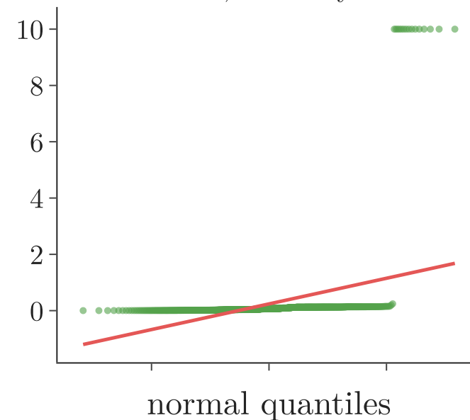
Reciprocal: 1 / (x + 0.1) skew 7.51, accuracy 61.7%
