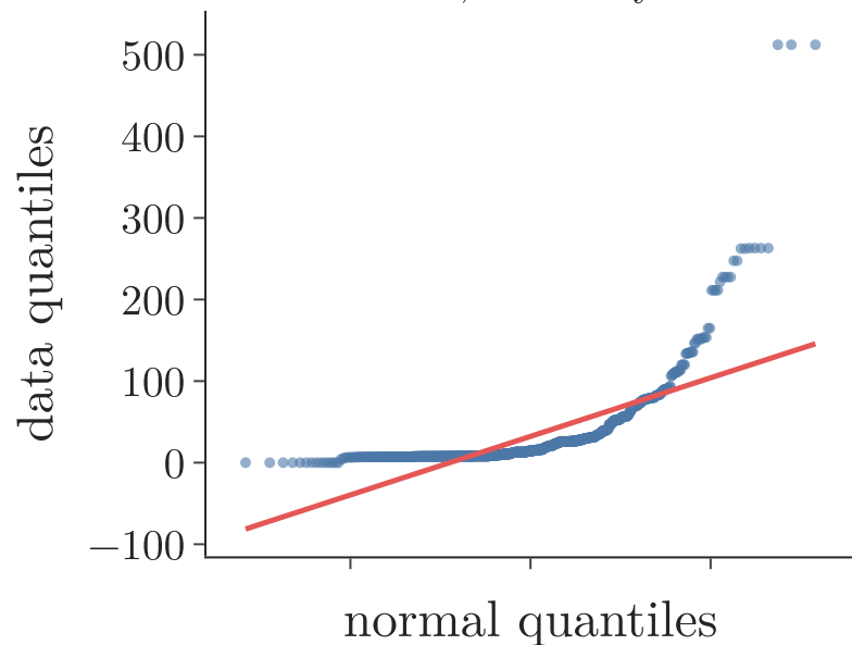
No transform skew 4.79, accuracy 65.9%
