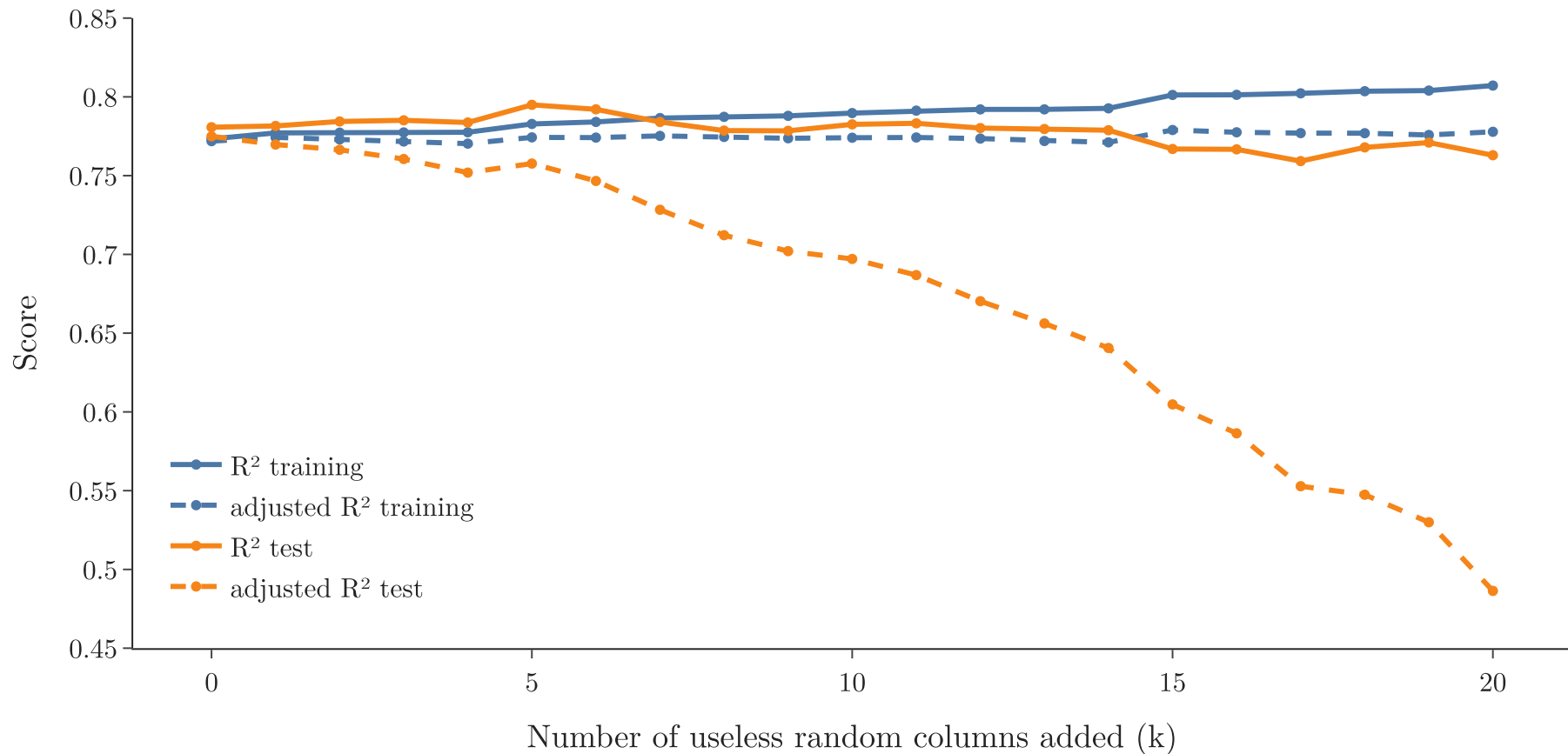
CGPA plus k columns of random numbers
