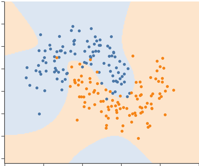
degree 4 (14 columns): CV accuracy 0.935
