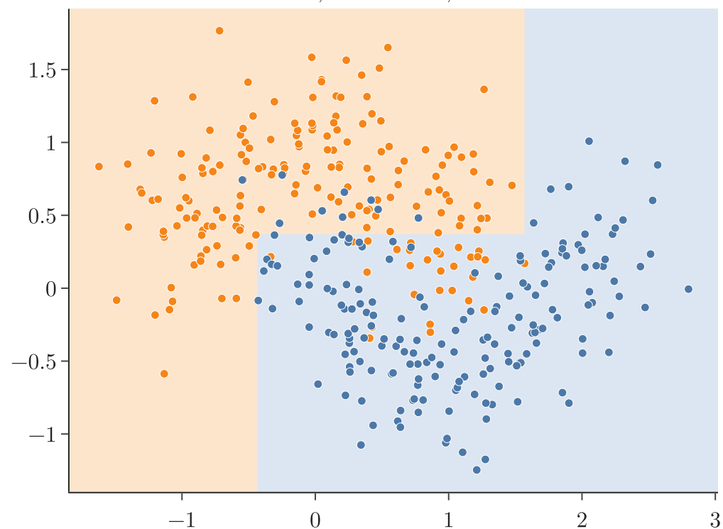
min_samples_split = 100 7 leaves, train 0.90, test 0.90
