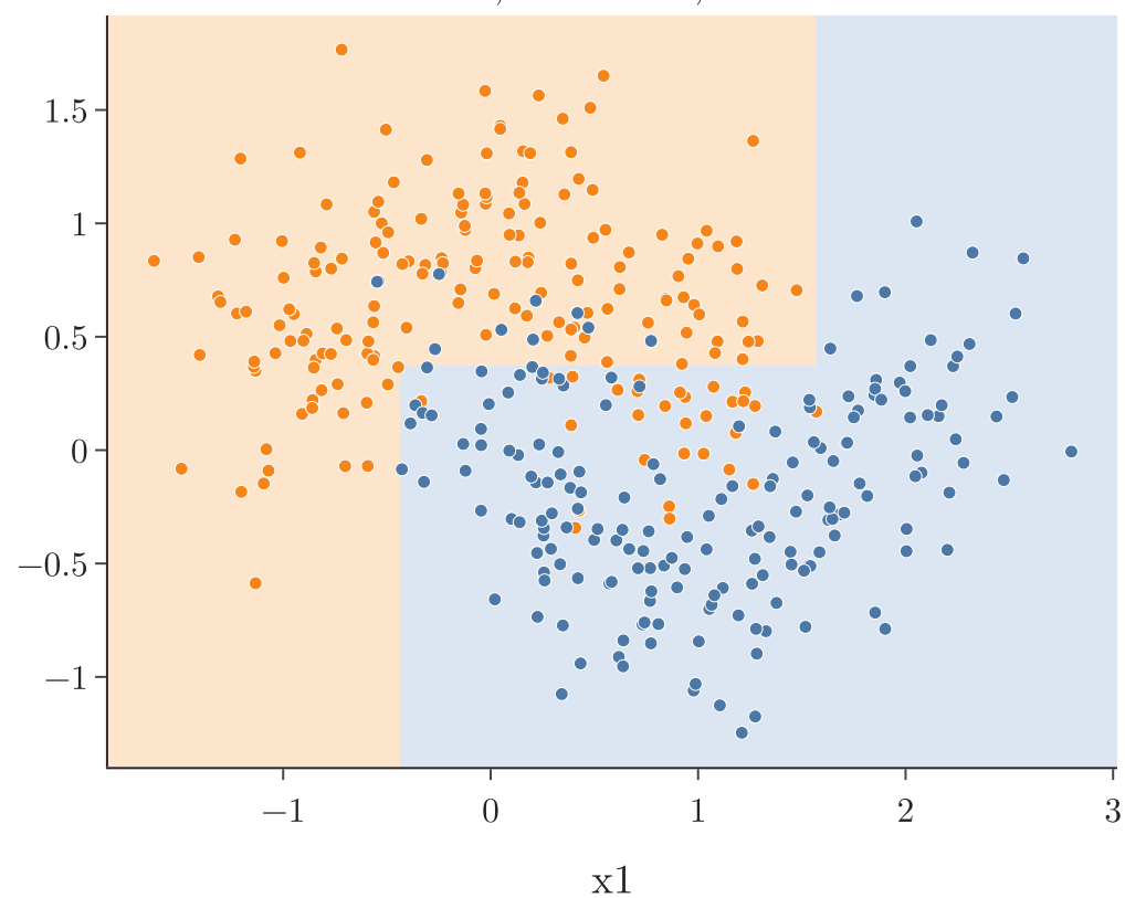
max_leaf_nodes = 5 5 leaves, train 0.90, test 0.90
