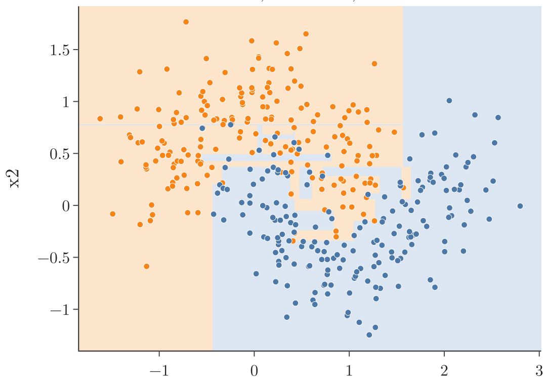
no limits (fully grown) 43 leaves, train 1.00, test 0.86
