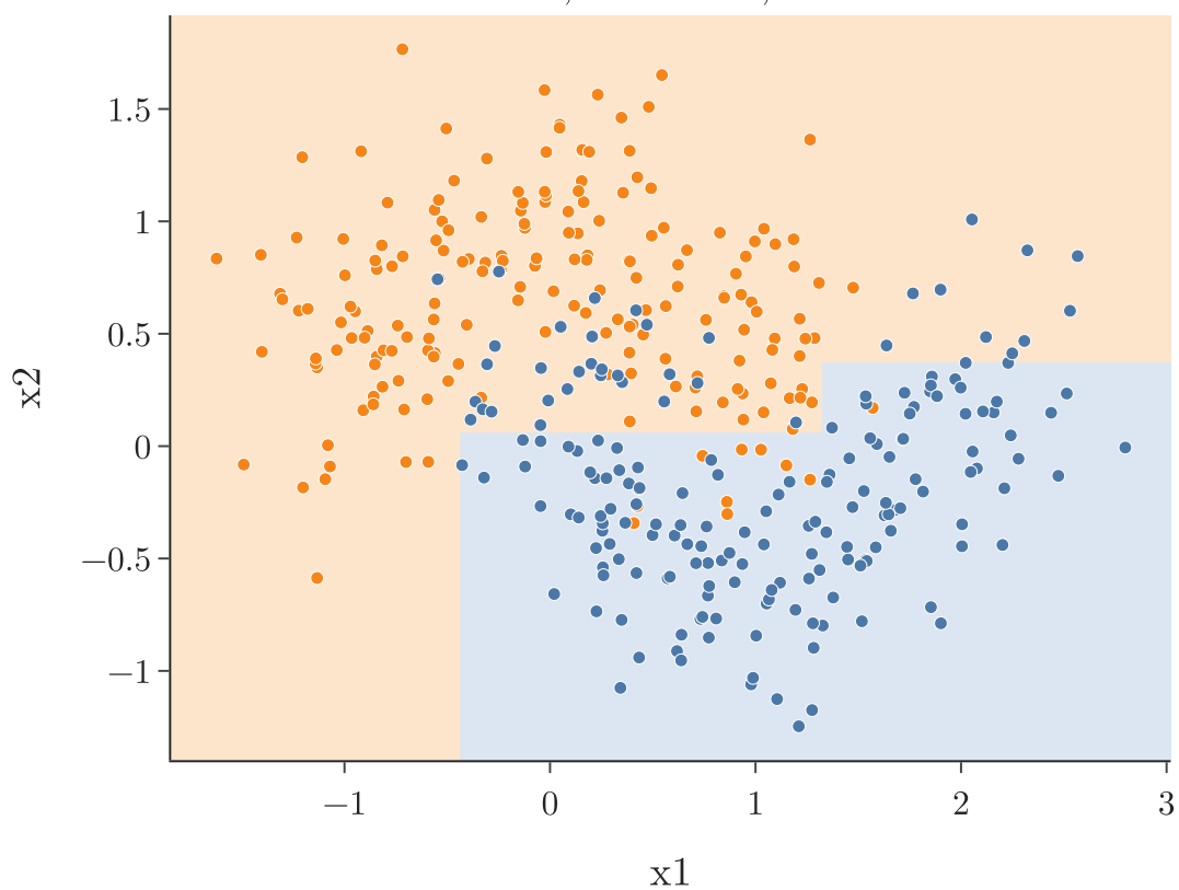
min_samples_leaf = 20 11 leaves, train 0.87, test 0.84
