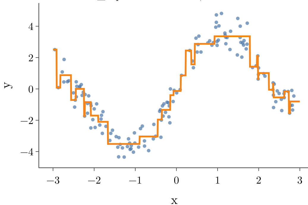
max_depth = 5: 30 leaves, test R^2 = 0.90
