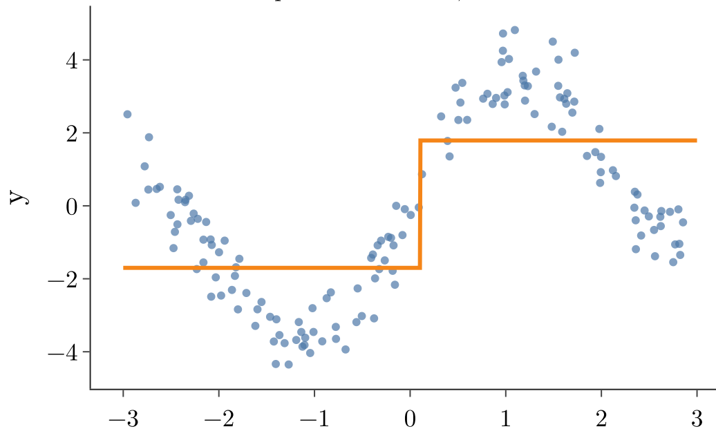
max_depth = 1: 2 leaves, test R^2 = 0.53
