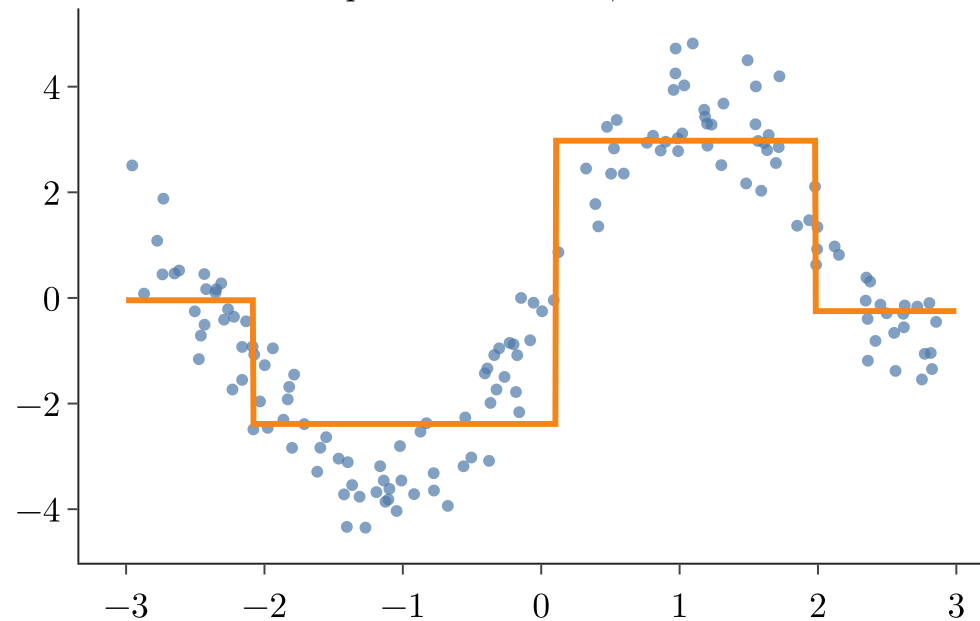
max_depth = 2: 4 leaves, test R^2 = 0.75
