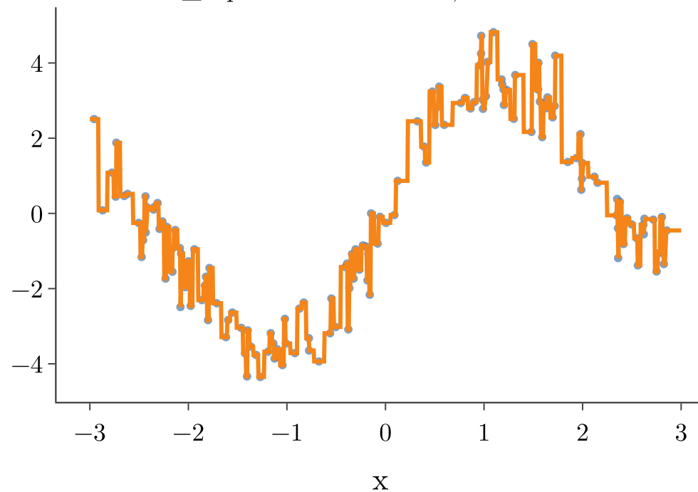
max_depth = 15: 149 leaves, test R^2 = 0.87
