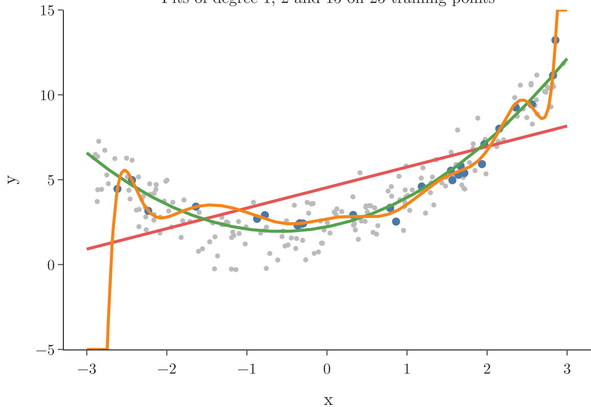
Fits of degree 1, 2 and 15 on 25 training points
