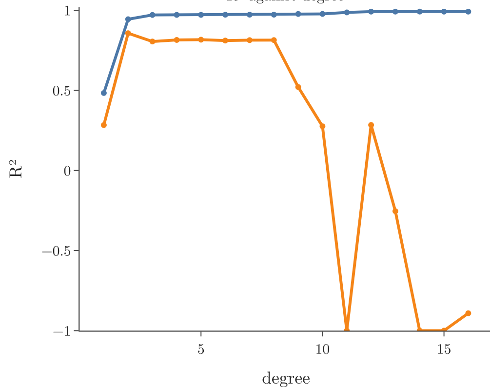
R^2 against degree
