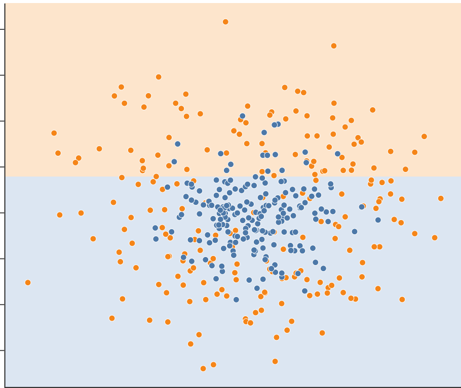
n_estimators=500, learning_rate=1.0 train 0.85, test 0.84
