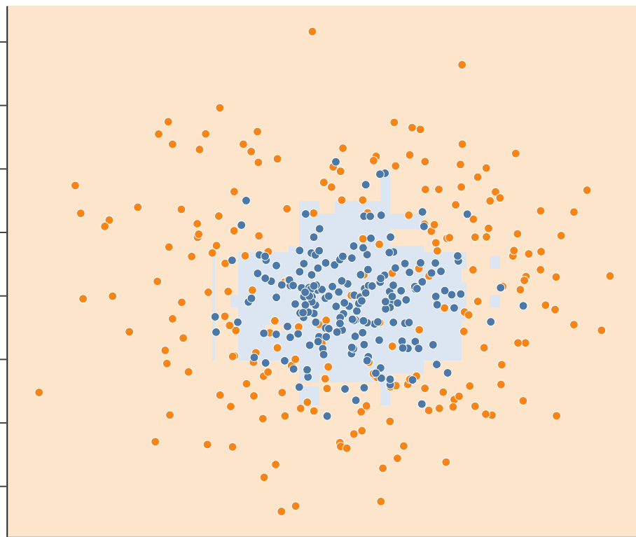
n_estimators=1500, learning_rate=1.0 train 0.87, test 0.85
