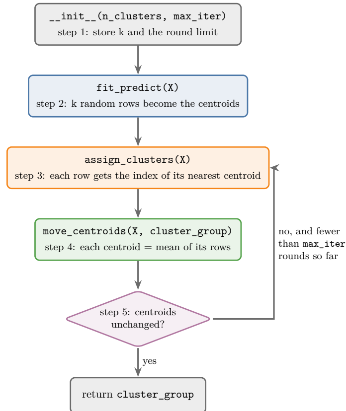
Figure 1: The KMeans class: which method does which step of k-means
