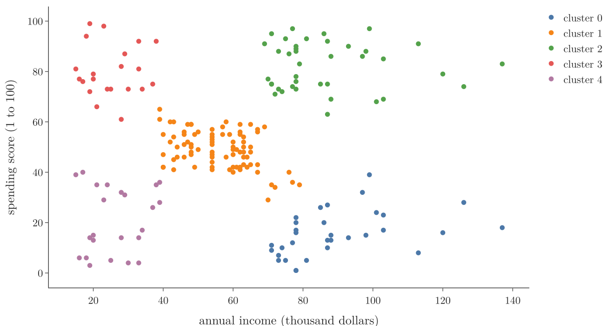
Figure 6: The 200 customers in the 5 clusters found by Ward linkage
