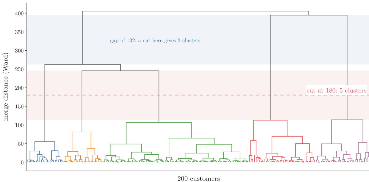
Figure 5: Ward dendrogram of the 200 customers; the cut at 180 gives 5 clusters
