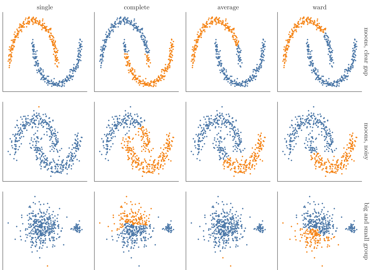
Figure 4: Single, complete, average and Ward linkage (2 clusters) on moons with a clear gap, noisy moons, and a big and a small group
