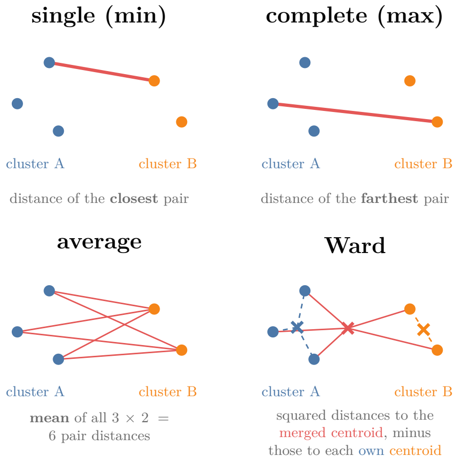
Figure 3: The four linkages: how the distance between cluster A and cluster B is measured
