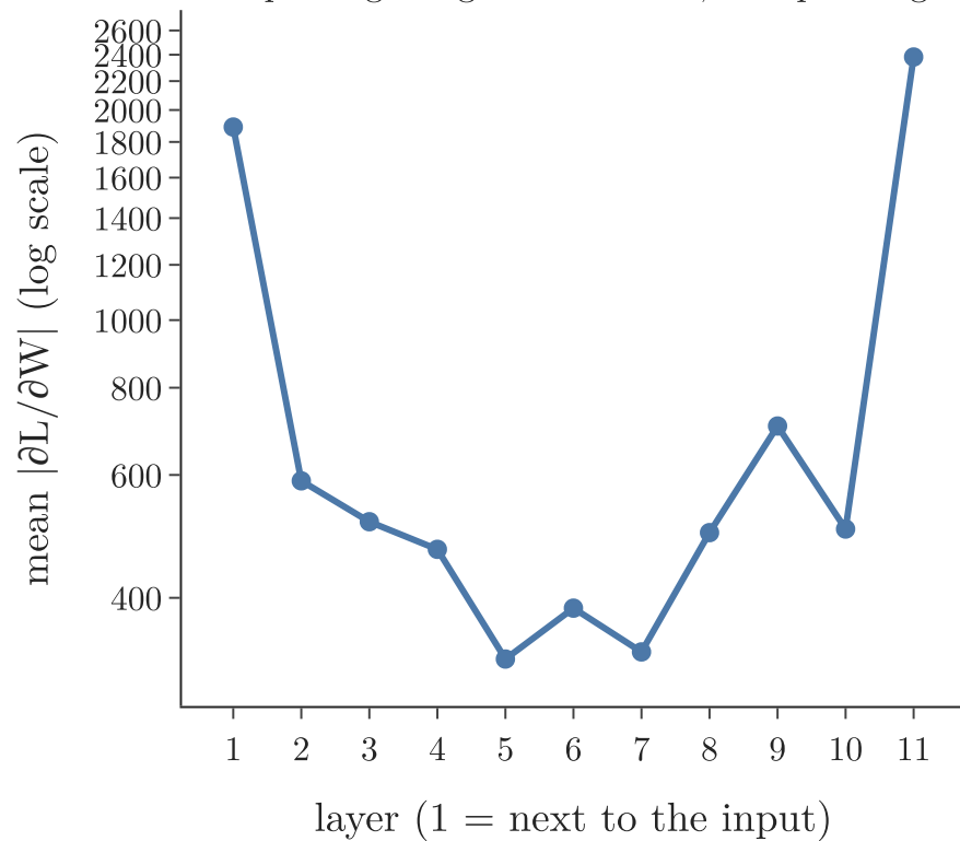
Exploding: weights with std 1, no squashing
