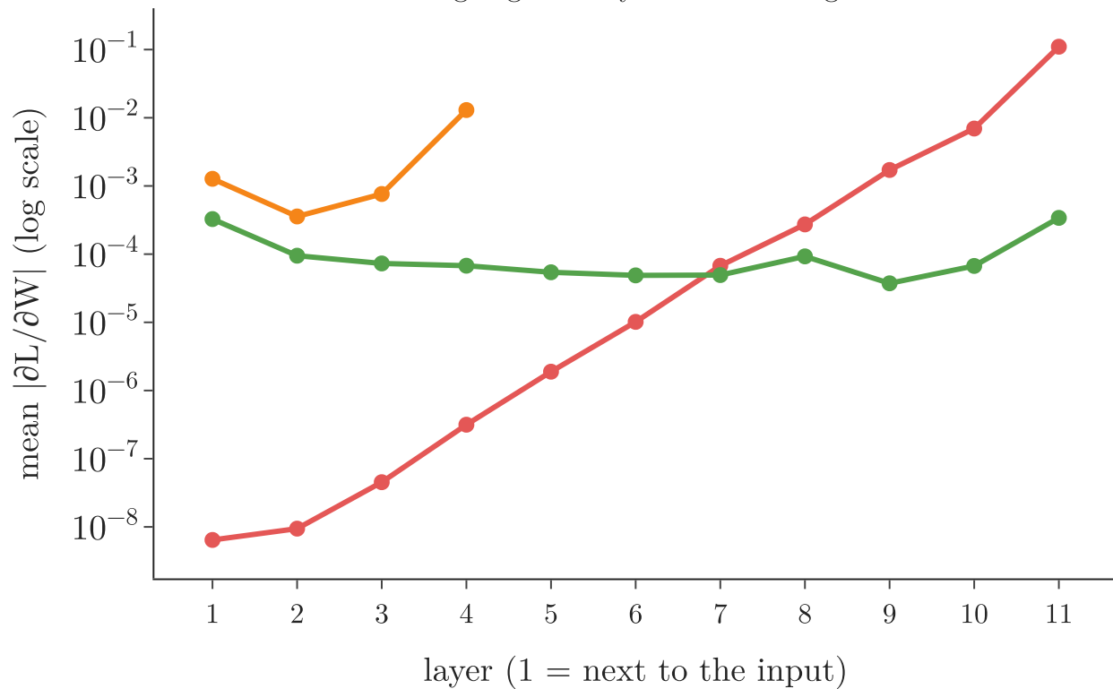
Vanishing: sigmoid layers shrink the gradient
