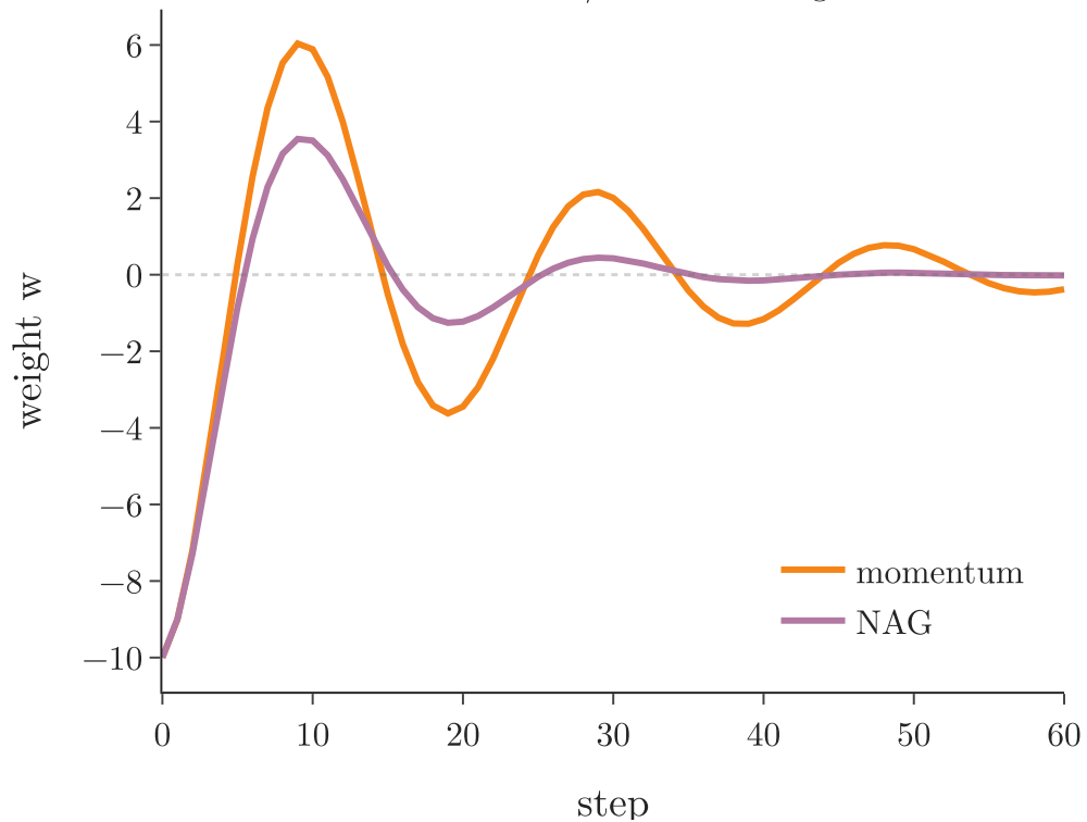
bowl L = w^2/2 : overshooting
