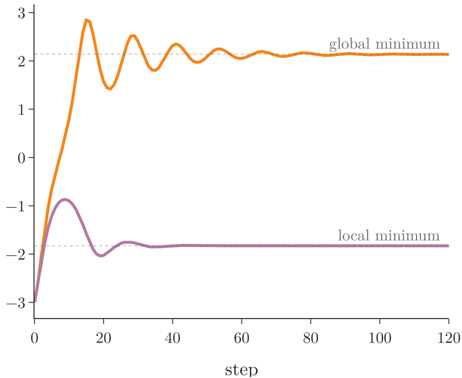
curve with a local minimum
