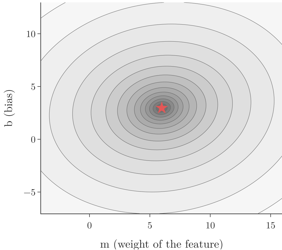
dense feature: round bowl
