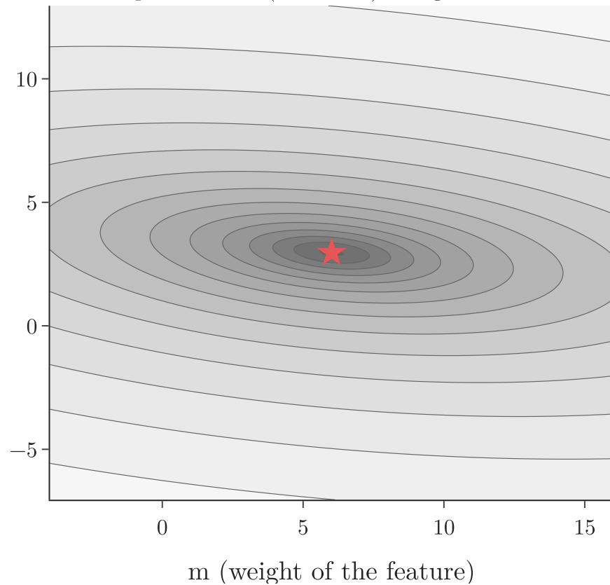
sparse feature (90% zeros): elongated bowl
