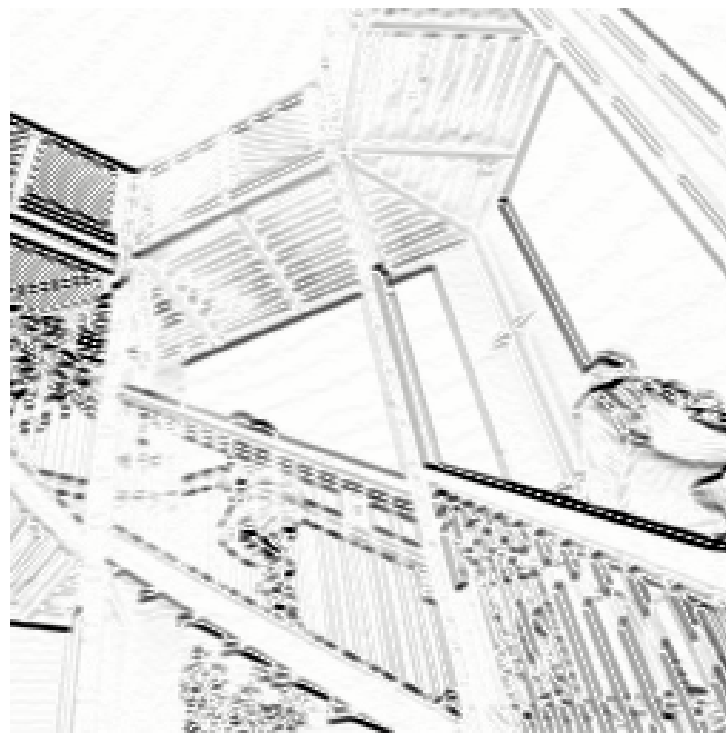
horizontal-edge filter
