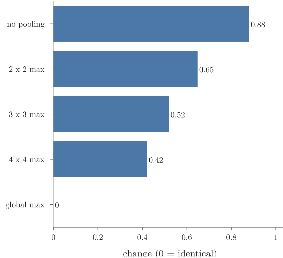
relative change after a 1-pixel shift
