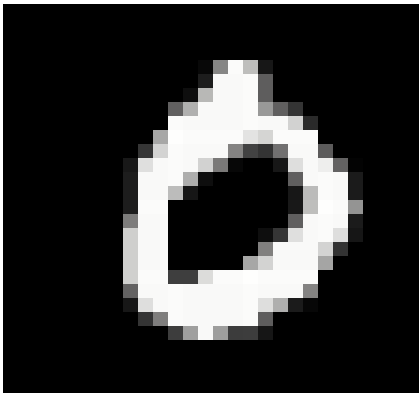
shifted 1 pixel
