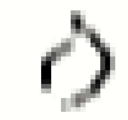
feature map
