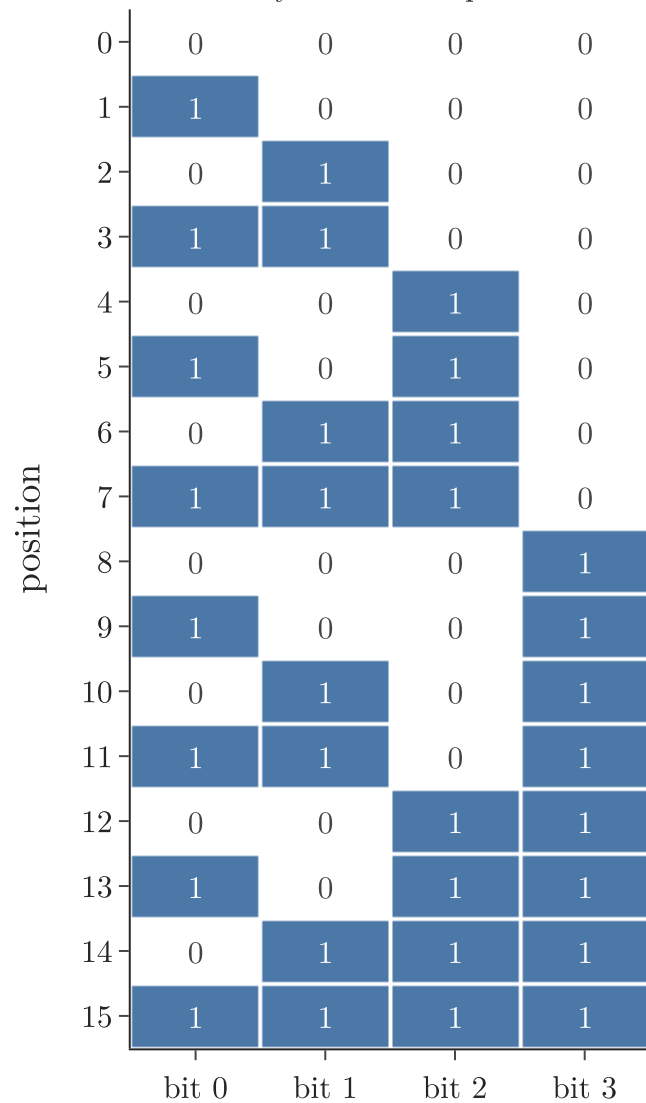
binary code of the position
