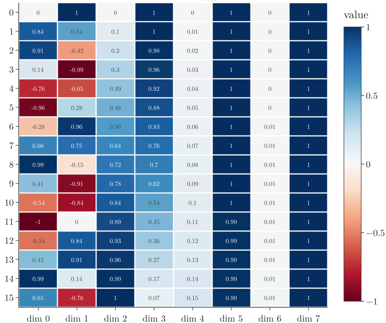
sine-cosine encoding, d_{\text{model}} = 8
