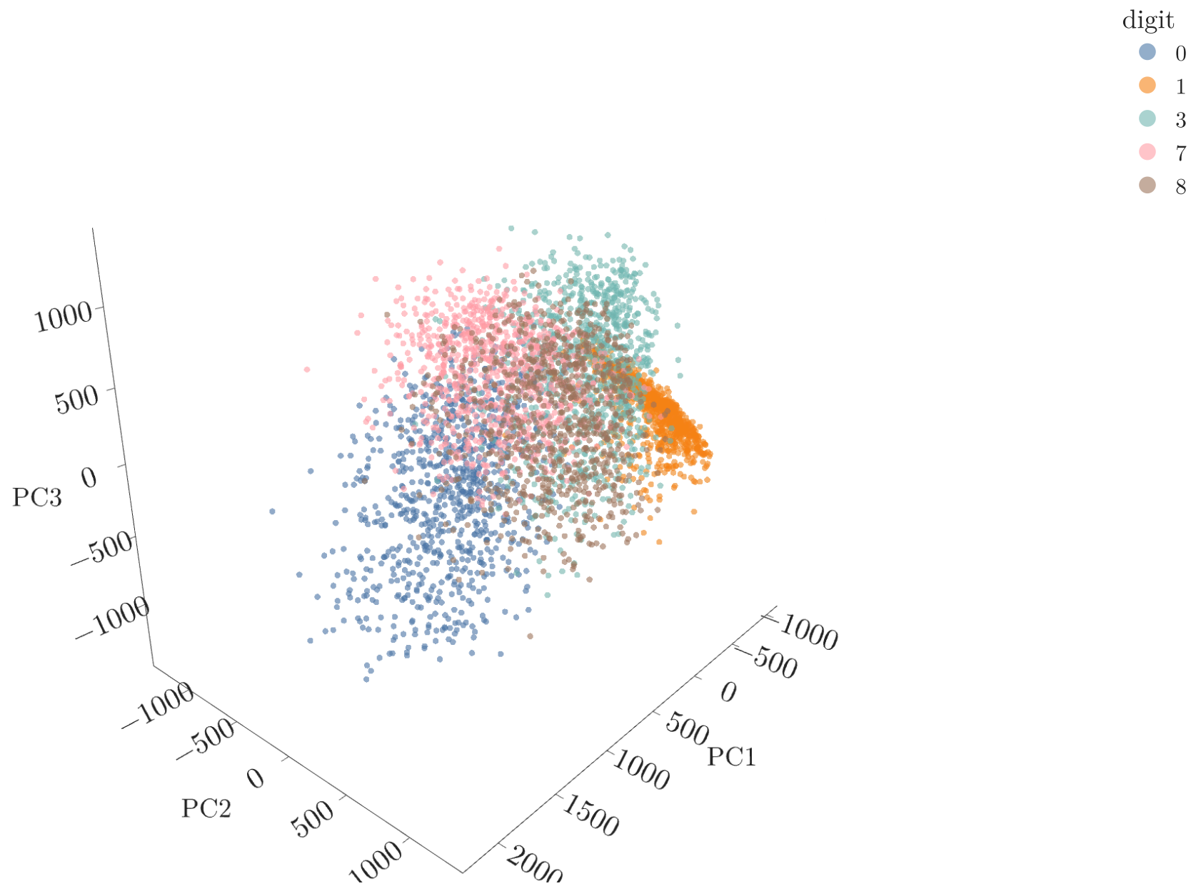
Digits 0, 1, 3, 7 and 8 on the first three principal components
