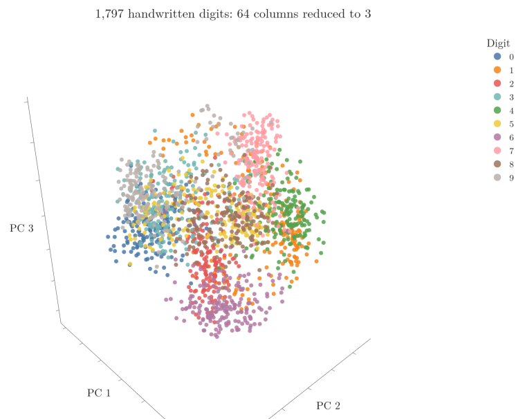
Figure 6: Handwritten digits: 64 features reduced to 3
