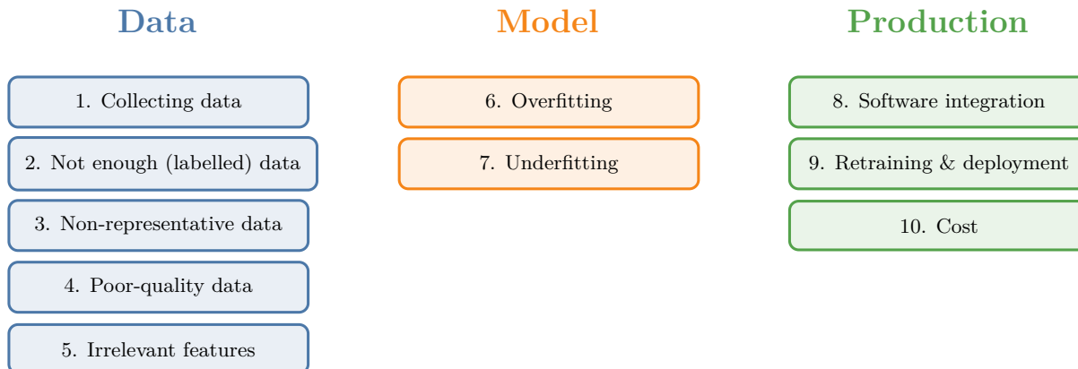
Figure 1: The ten main challenges in ML
