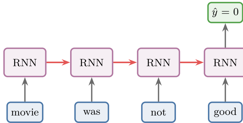
Figure 1: Many-to-one, unrolled: one word enters at each time step, the hidden state passes to the next step (red arrows), and only the last step produces an output
