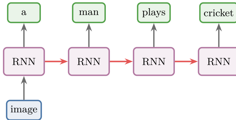
Figure 2: One-to-many, unrolled: the image enters at the first time step only; every time step produces one word of the caption
