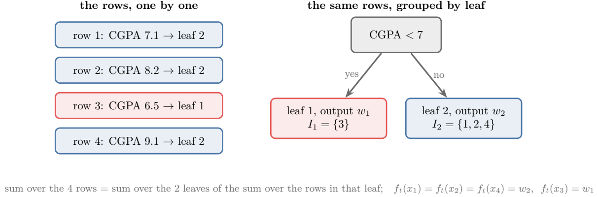
Figure 4: Four observations and a tree with two leaves: adding up the observations one by one gives the same total as adding them up leaf by leaf
