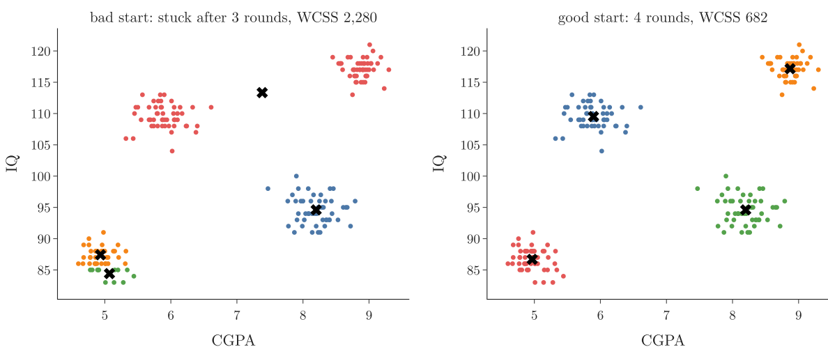
Figure 3: The same students and k = 4 from two random starts: stuck in poor clusters (left) and the right clusters (right)
