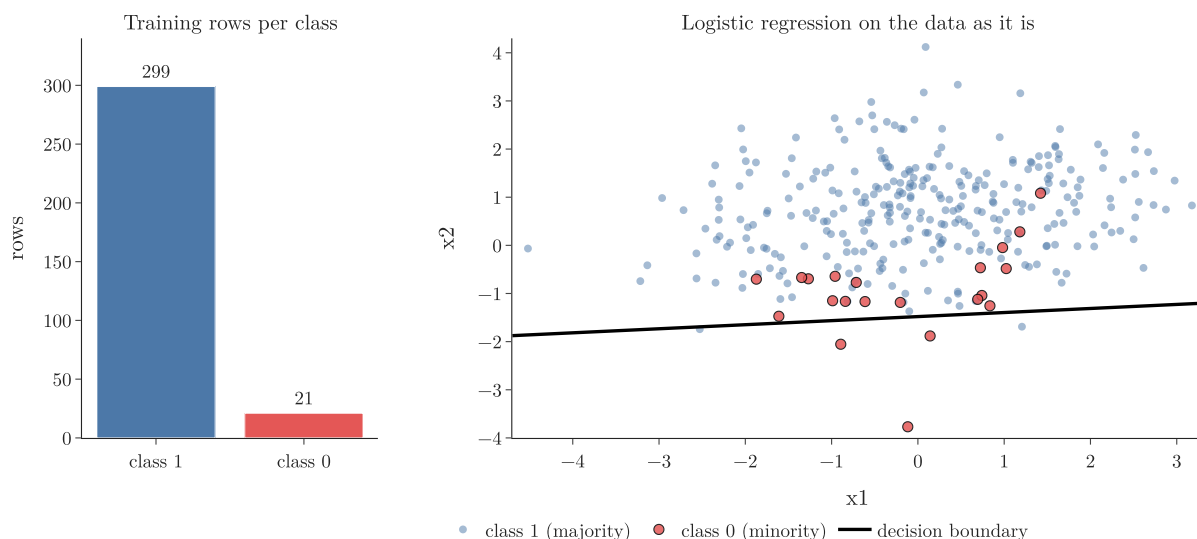
Figure 2: Left: the training observations per class. Right: the line logistic regression learns on this data
