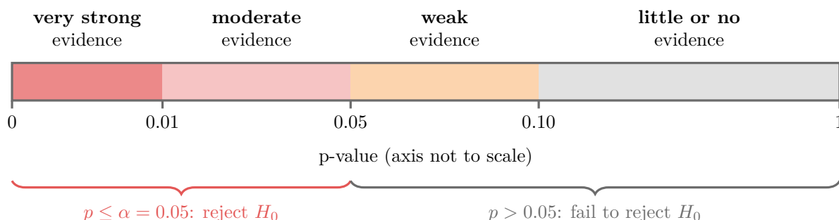
Figure 2: A common rule of thumb for reading p-values
