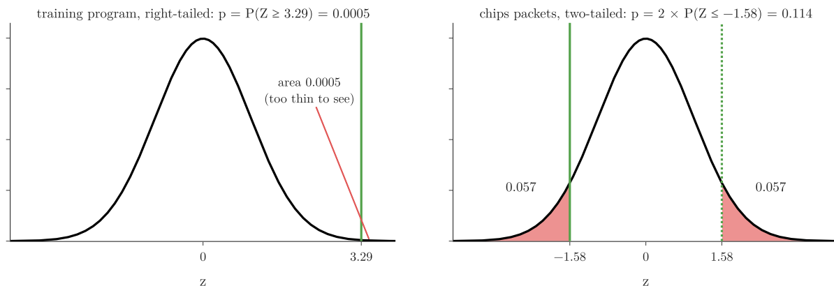
Figure 3: P-values (red areas) of the two z-tests
