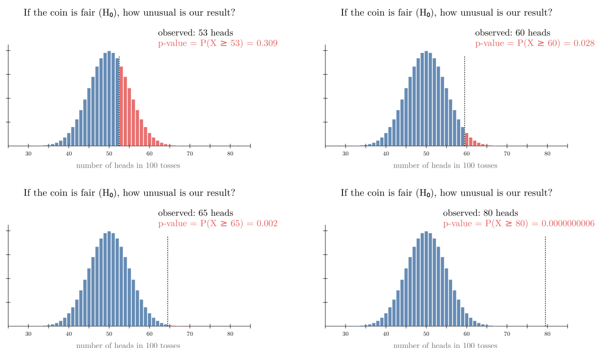
Figure 1: P-value of 100 coin tosses under H_0 (fair coin): the red bars, at or beyond the observed number of heads, add up to the p-value
