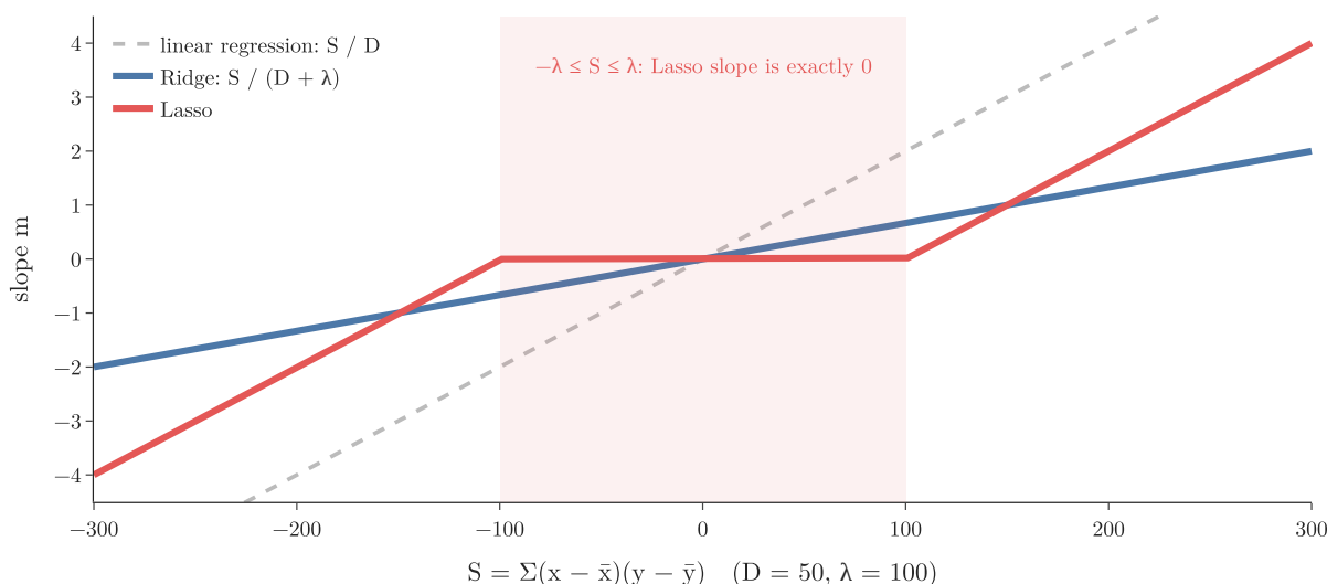
Figure 2: The slope against S for linear regression, Ridge and Lasso
